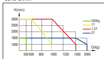
LOAD CHART
